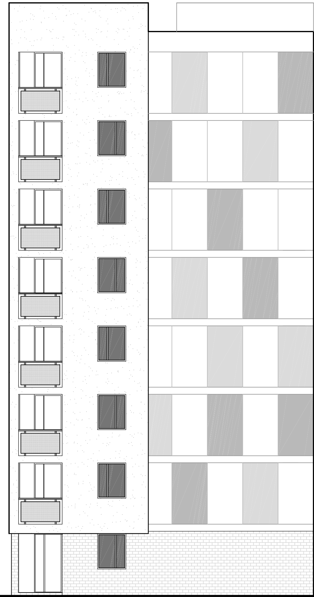
North elevation
